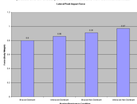
Figure 3. Lateral Peak Impact Force (LPIF), as a unit of BW, in two experimental conditions (braced and un-braced) and on dominant and non-dominant ankles.
